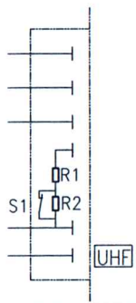
Wiring diagram
