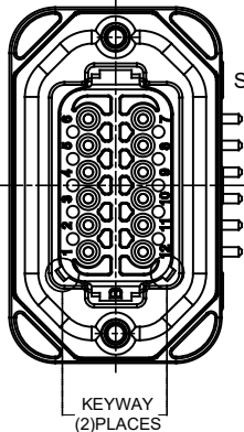
P/N AT13-12PB-BMXX KEY-B CONFIGURATION STANDARD COLOR: BLACK
