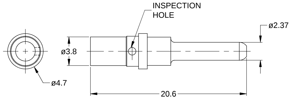
REFERENCE DIMENSIONS
