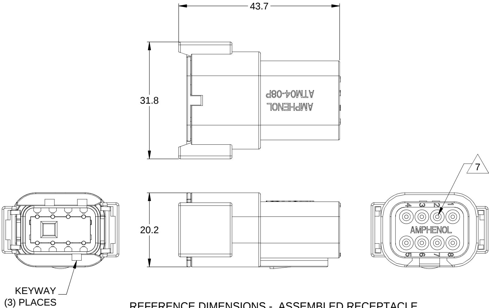
REFERENCE DIMENSIONS - ASSEMBLED RECEPTACLE
