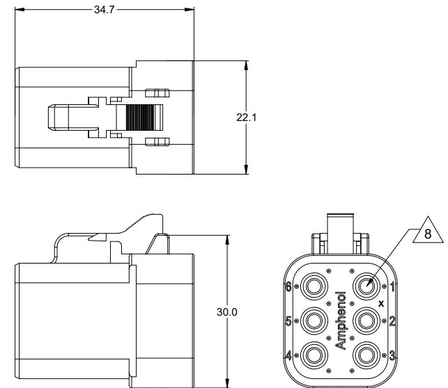
REFERENCE DIMENSIONS - ASSEMBLED PLUG
