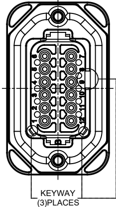
P/N AT15-12PB-BM1X KEY-B CONFIGURATION STANDARD COLOR: BLACK
