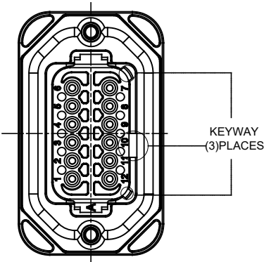
P/N AT15-12PA-BM1X KEY-A CONFIGURATION STANDARD COLOR: GREY
