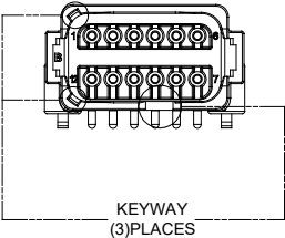
P/N ATF13-12PB-BM0X KEY-B CONFIGURATION STANDARD COLOR: BLACK
