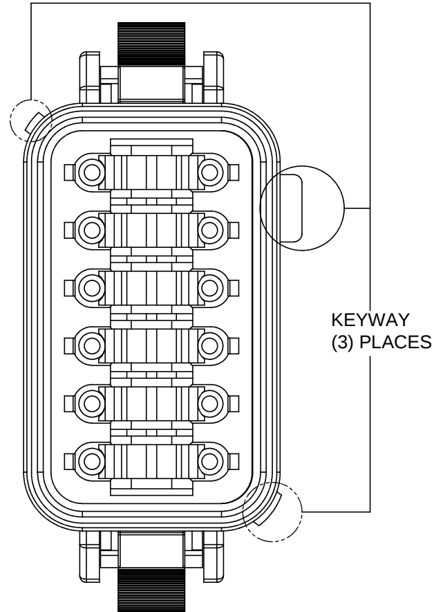
P/N AT06-12SD KEY-D CONFIGURATION STANDARD COLOR: BROWN
