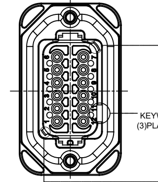
AT15-12PD-BM1X VARIANTS
