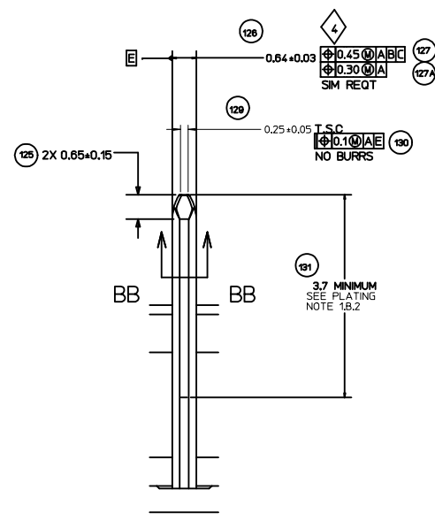
SECTION U-U TYPICAL
