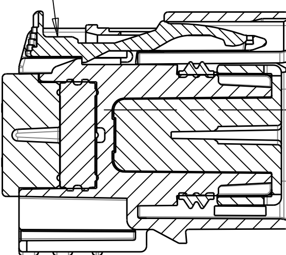
SECTION B-B (RECEPTACLE INSERT SHOWN IN FULL-LOCK) SEE NOTE #2
