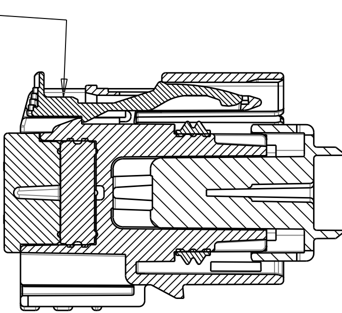
SECTION B-B (RECEPTACLE INSERT WITH SHORTING BAR LIFTER SHOWN IN PRE-LOCK) SEE NOTE #2
