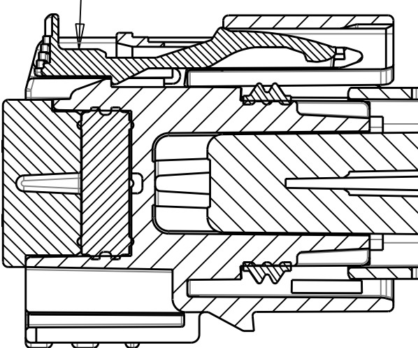
SECTION B-B (RECEPTACLE INSERT SHOWN IN PRE-LOCK) SEE NOTE #2
