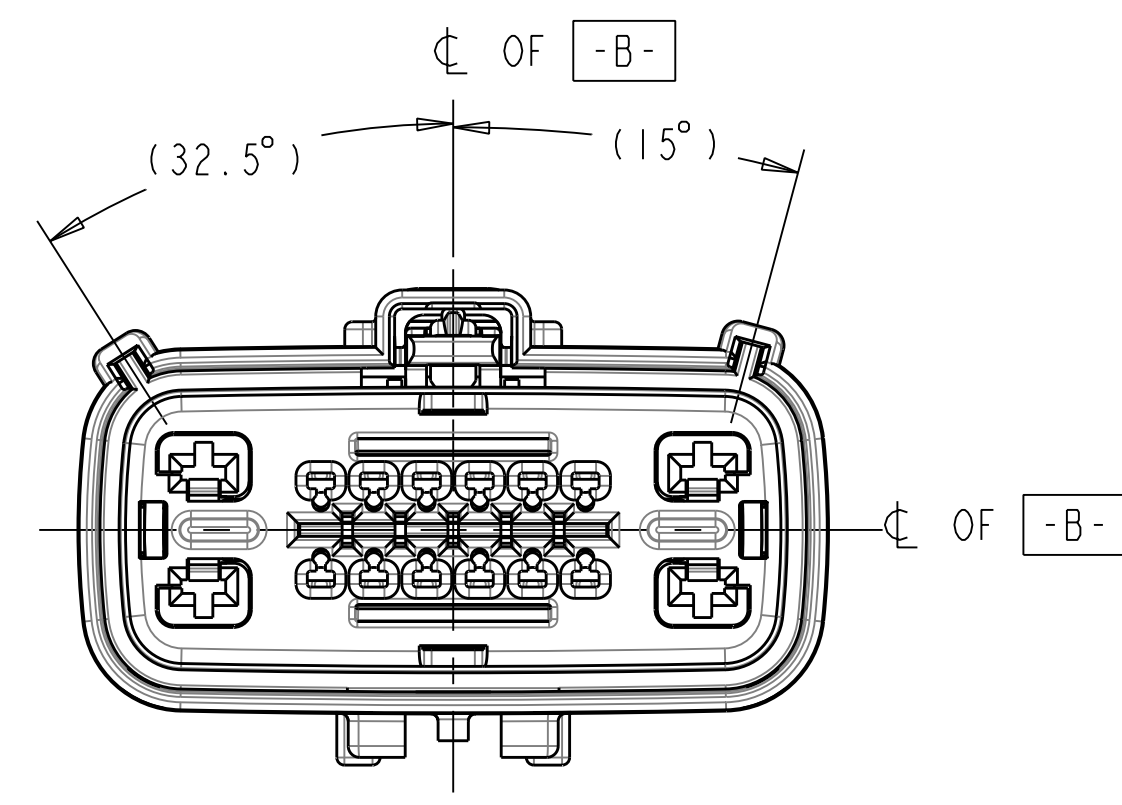
KEYING OPTION F SCALE 2:1
