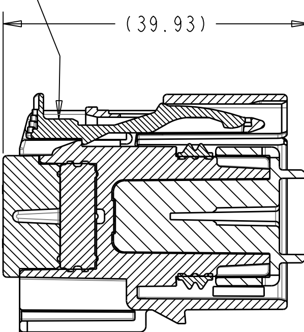
SECTION B-B (RECEPTACLE INSERT WITH SHORTING BAR LIFTER SHOWN IN FULL-LOCK) SEE NOTE #2
