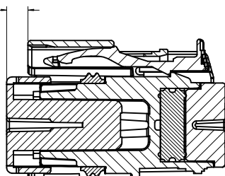
PRIMARY LOCK REINFORCEMENT (PLR) SHOWN IN PRE-STAGED POSITION SECTION X-X
