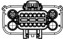
STANDARD (STD) - BLOCKED 2.8mm CAVITIES WITH CLIPSLOT
