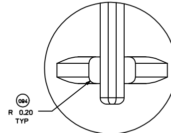
VIEW L
