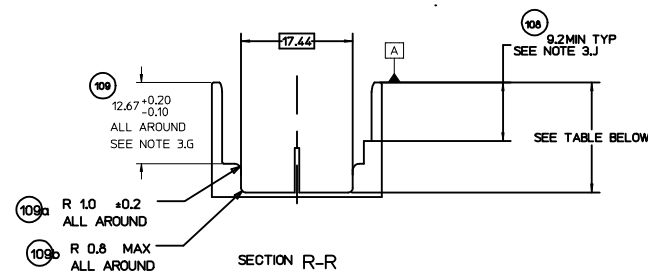
SECTION R-R
