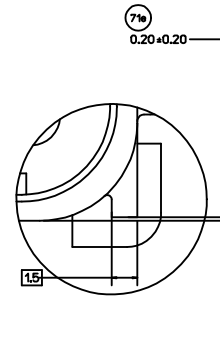
VIEW AE KEY TYPE 1
