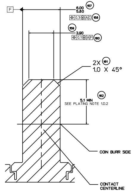
SECTION CB-CB
